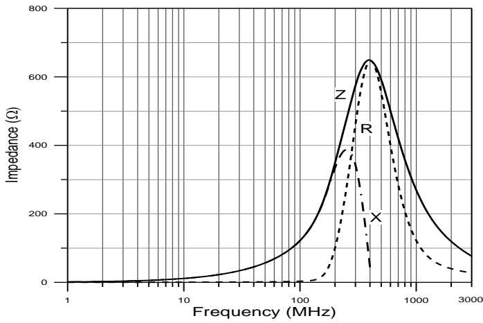
CME- NMCB160808H-121
